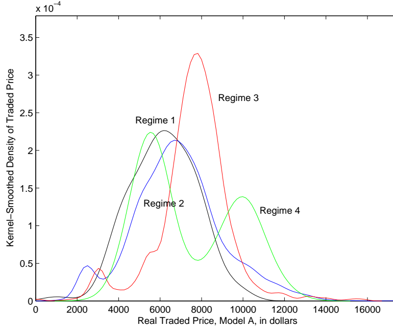
FIG 5. Estimated Kernel-Smoothed Densities of Traded Prices—Mid-Sized, Model A
